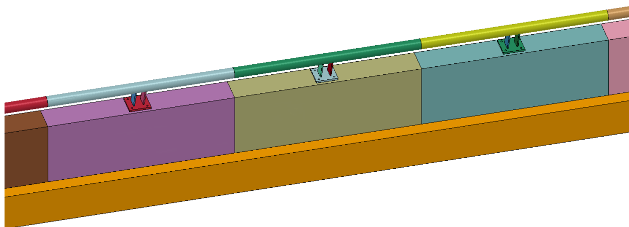
Figure 3.6 Barrier nos 7, 8, and 9 after the impact
